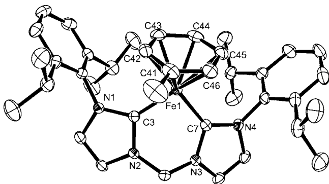
Figure 4. ORTEP representation of 3 ·Et 2 O in the solid state at 50% probability. H atoms omitted for clarity, in addition to the cocrystallized Et 2 O molecule. Selected bond lengths [Å]: Fe1–C3 1.9190(19), Fe1–C7 1.9212(19), Fe1–C42 2.096(2), Fe1–C41 2.096(2), Fe1–C43 2.107(2), Fe1–C46 2.114(2), Fe1–C44 2.118(2), Fe1–C45 2.135(2), C41–C46 1.409(3), C41–C42 1.422(3), C42–C43 1.410(3), C43–C44 1.407(3), C44–C45 1.413(3), C45–C46 1.406(3). Selected bond angle [°]: C3–Fe–C7 89.36(8).
