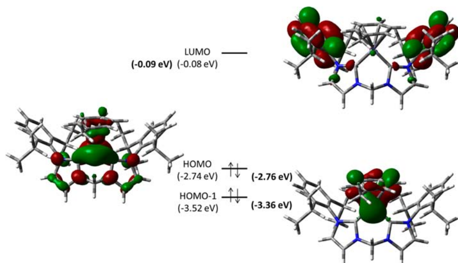
Figure 7. Boundry surfaces of the calculated frontier molecular orbitals in complex 3. The energies in bold parentheses are the calculated energies for the corresponding MOs in complex 4 which are comparable.
