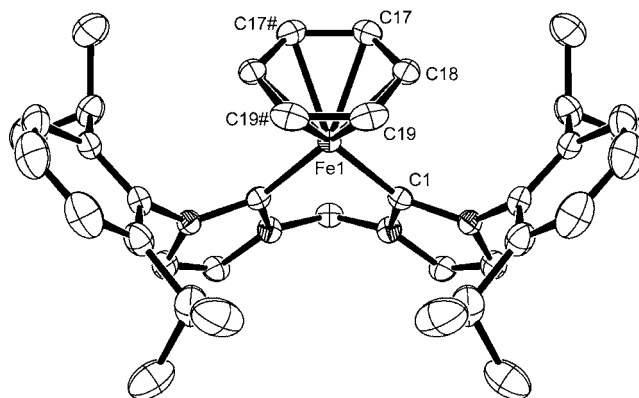
Figure 5. ORTEP representation of 4 in the solid state at 50% probability. H atoms omitted for clarity. (Symmetry transformations used to generate equivalent atoms #: 1 - x + 2, y, z ). Selected bond lengths [Å]: Fe1–C1 1.921(3), Fe1–C19 2.119(3), Fe1–C17 2.121(3), Fe1–C18 2.125(3), C17–C17# 1.404(6), C17–C18 1.405(4), C18–C19 1.416(5), C19–C19# 1.385(7). Selected bond angle [°]: C1–Fe1–C1# 88.92(16).
