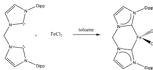
Scheme 1. Synthesis of 1 by Coordination of \{(\text{DippC:})_2\text{CH}_2\} to \text{FeCl}_2
